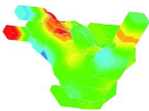
Acoustic modes of an air conditioning module
