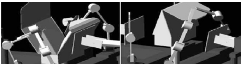
Figure 9. Carton folding simulation matches real-life robot [14]
