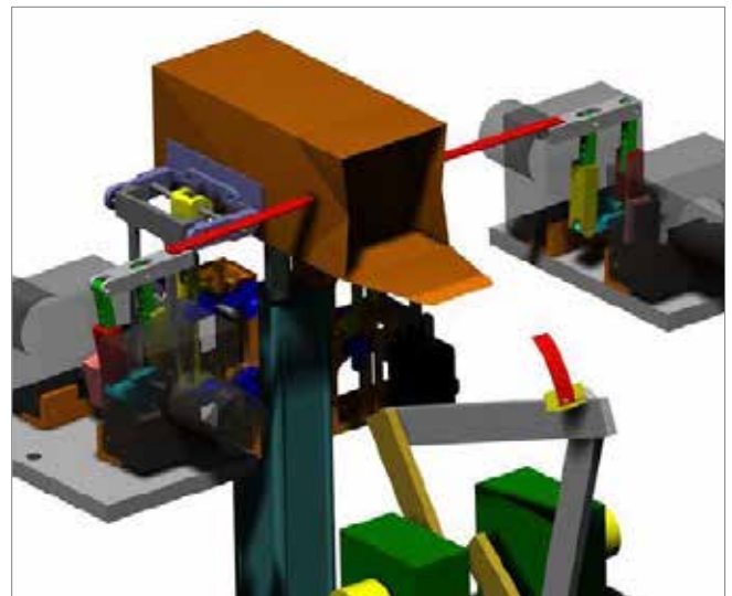
3D Adams simulation for package folding machinery
