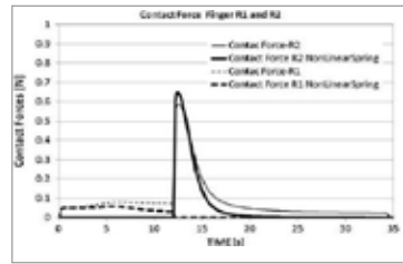
Figure 9. Finger contact force from simulation [2].
