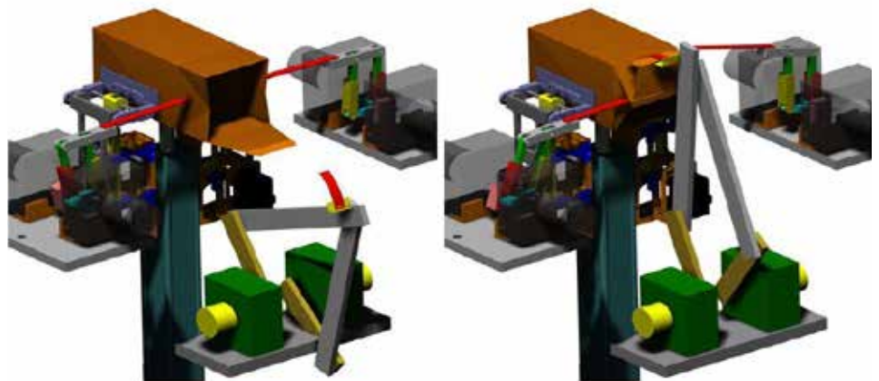
Figure 3. 3D Adams simulation for package folding machinery
