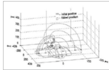
Figure 6. Carton folding trajectories for more complex folding operation [13]
