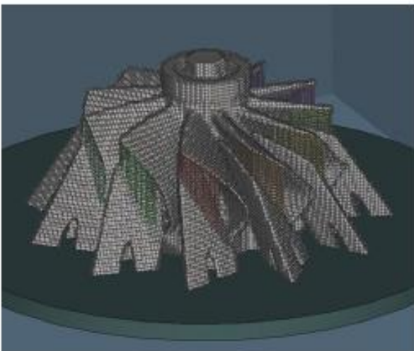
Image 1: Simulation helps to reduce component distortion and thus to keep tight tolerances.
