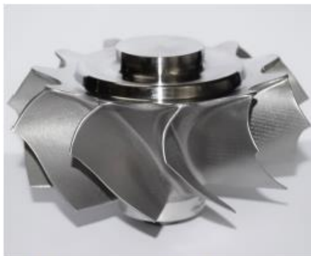
Image 2: From design to simulation to the finished component – less distortions thanks to Simufact Additive.
